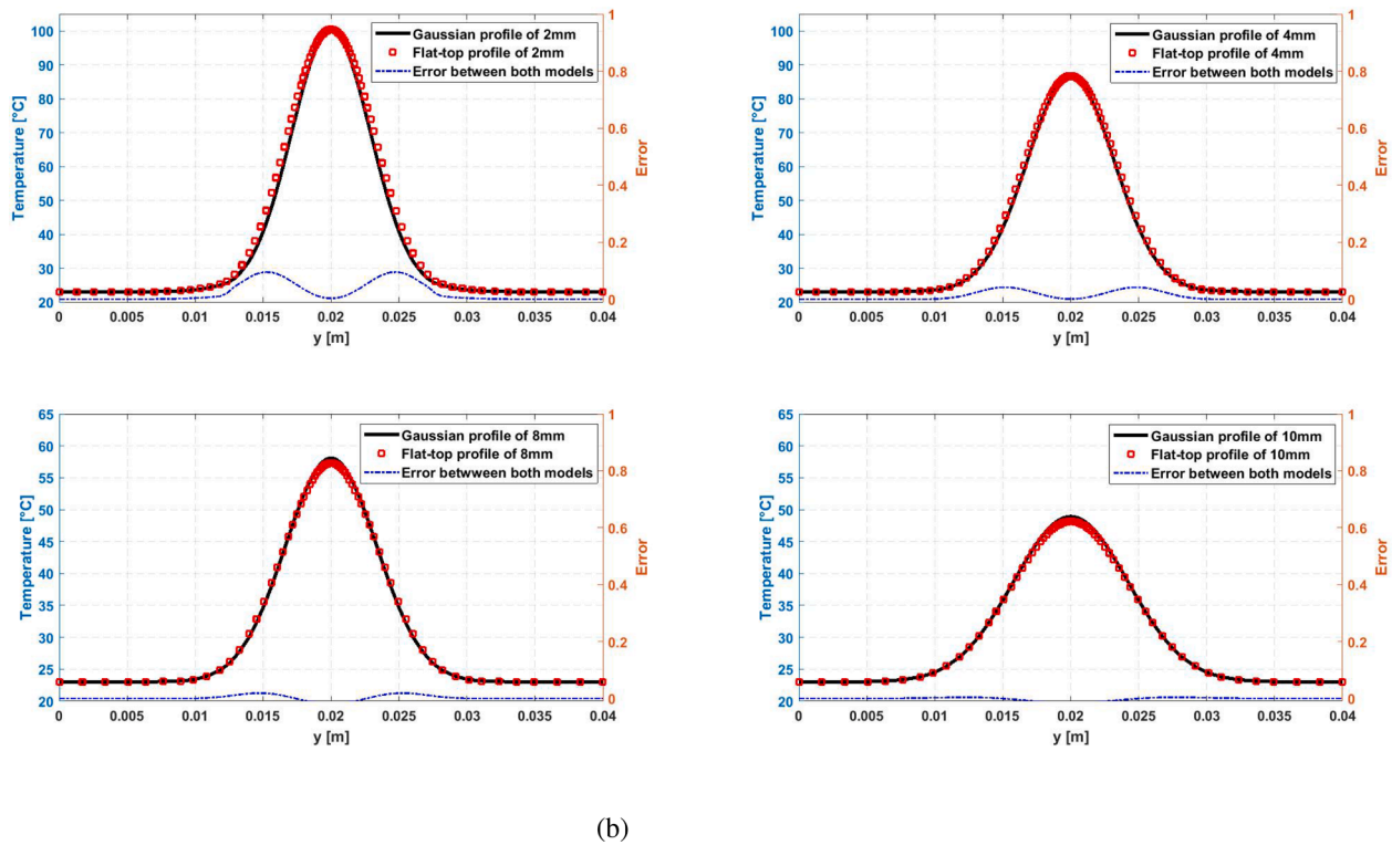
Fig. 18. Distribution and comparison of the profile of maximum temperature without scattering effect for both samples of 2 mm and 10 mm (b) Comparison of the profile of maximum temperature for two types of energy distribution.
