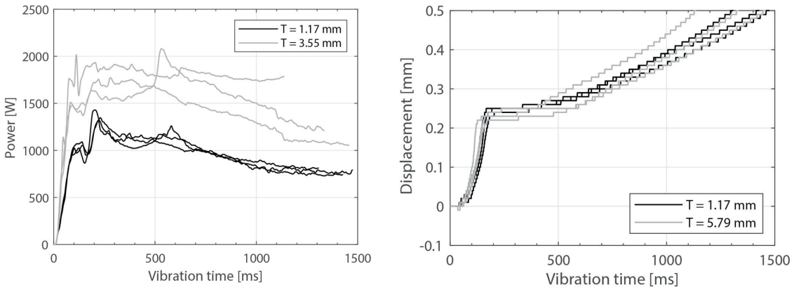
Figure 9. Consumed power (left) and downward displacement (right), three repetitions for two bottom adherend thickness values. The welding parameters were 500 N force and 80 \mu m vibration amplitude. The top adherend’s thickness was 1.83 mm.
