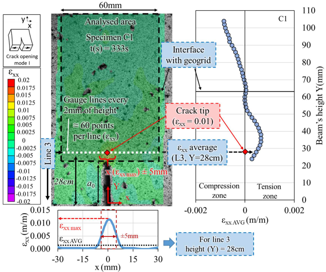
2 Figure 6. Explanation of procedure of analysis performed with Digital Image Correlation (DIC) 3 technique (specimen C1, t=333s)
